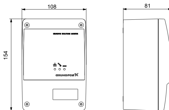
Front view (left), side view (right)
